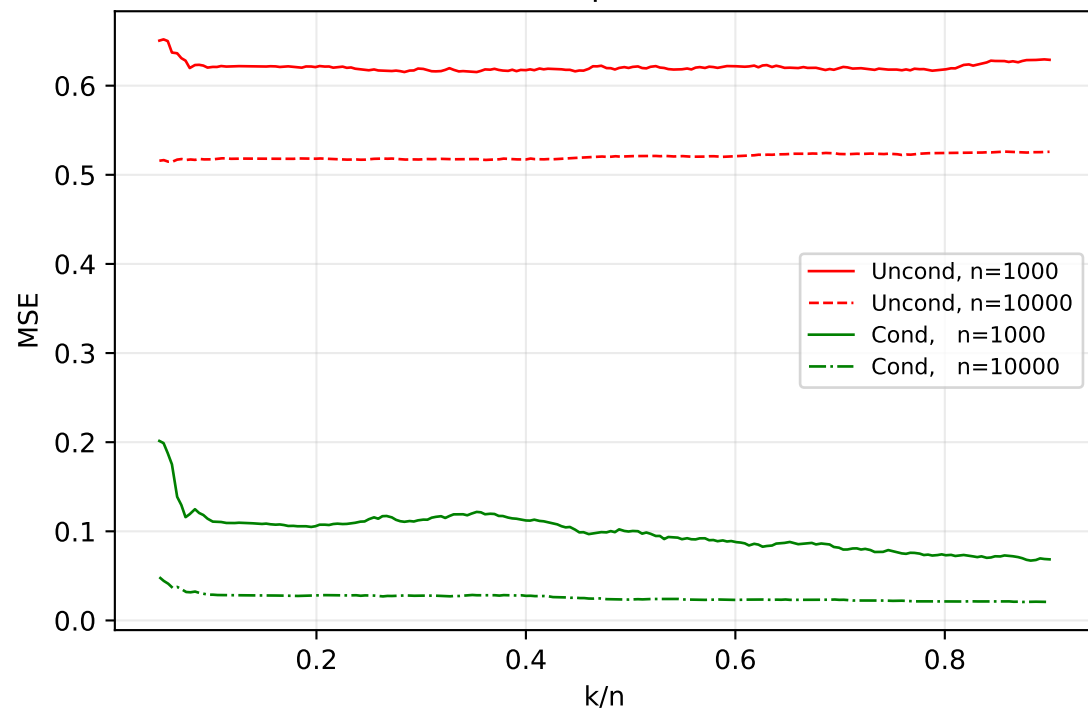
MSE, q = 0.95
