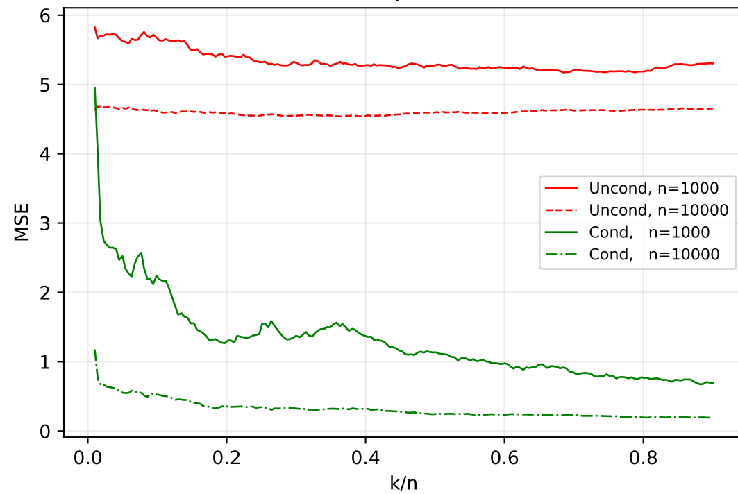
MSE, q = 0.99
